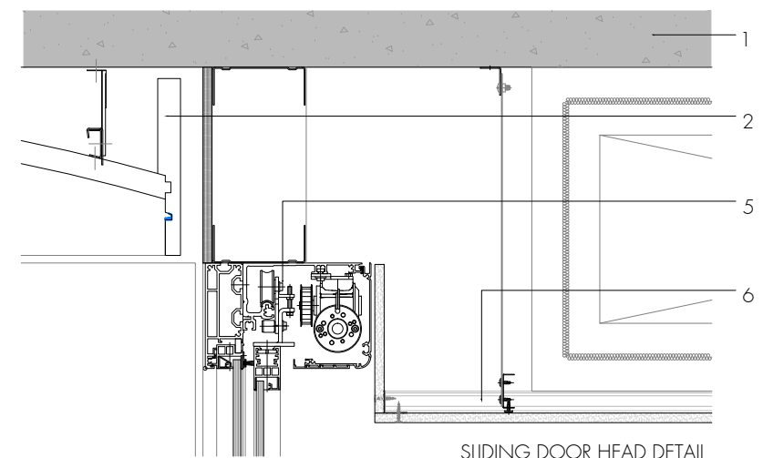
SLIDING DOOR HEAD DETAIL
